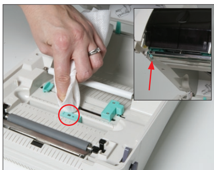
7. Remove dust or paper particles from the 'media' sensor and 'cover open' sensor using a dry Toshiba Cleaning Cloth.
